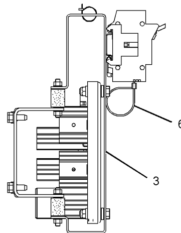
VIEW B-B
